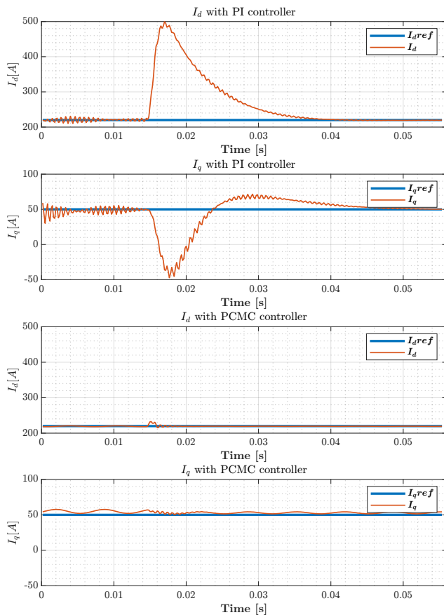
Fig. 8. Response of the two control approach to 30 % grid voltage drop
