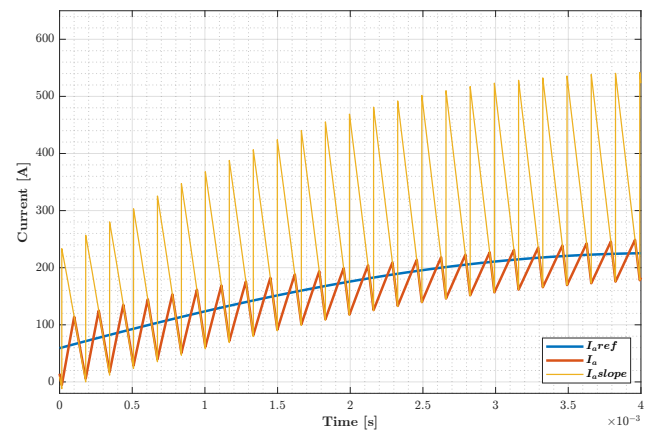
Fig. 5. Measured, reference and compensated reference phase current of the PCMC simulation
