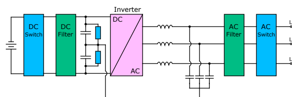
Fig. 1. The block diagram of the grid-connected energy storage system
