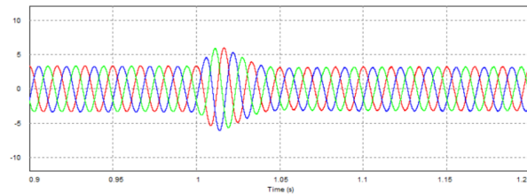
Fig. 14. VI response for a grid frequency drop of 0.1 Hz
