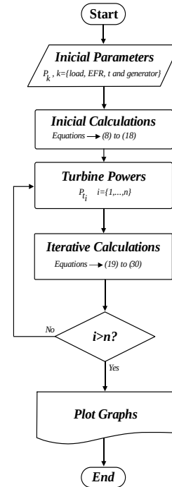
Fig. 7. A simplified flowchart logic algorithm for to analyzing the influence of pole numbers for the EFR and inductance generator.
