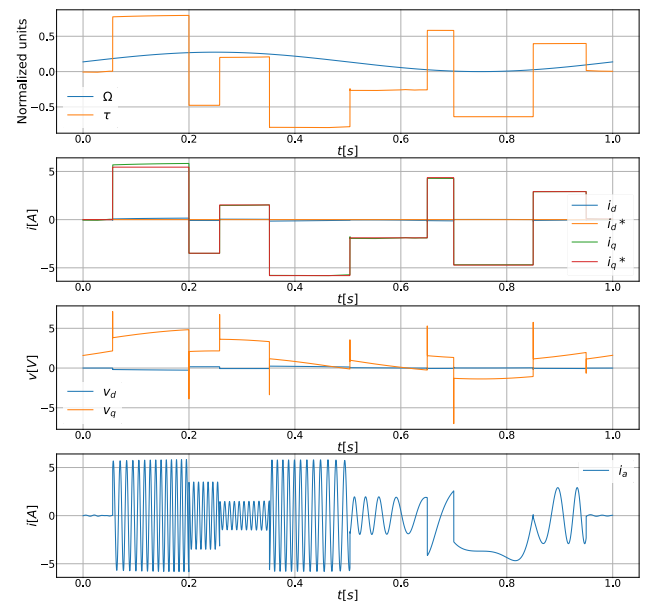
Fig. 7. Trajectories of the MATLAB RL Agent controlled PMSM motor with an outer speed control
