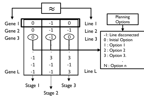
Fig. 3. Chromosome Encoding.
