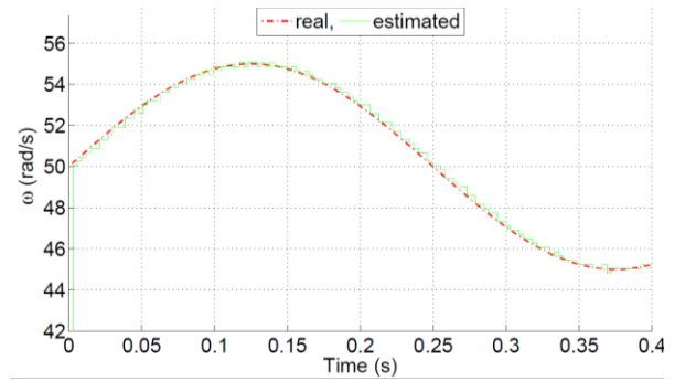
Fig. 1. Mechanical speed and its estimation using the conventional method with T_\omega = 3 ms.
