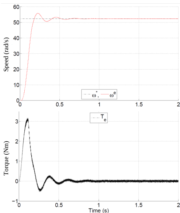
Fig. 4. Trajectories of speed (top) and torque (bottom) for a step test using tuning T2.
