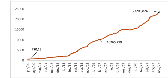
Fig. 2. Installed Capacity in Megawatts (MW) - Brazil from 2010 to 2022, monthly data. Source: Own elaboration based on the analyzed data.
