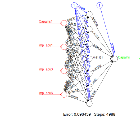
Fig. 3. Artificial Neural Network – Configuration ( net_{1t} ) (Equation 1) Source: own elaboration
