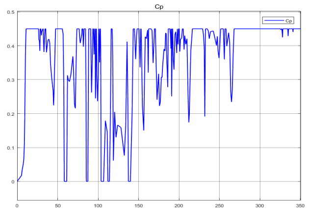
Fig. 8. Power coefficient C_p
