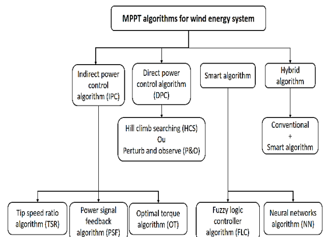
Fig. 6. Classification of different MPPT algorithms
