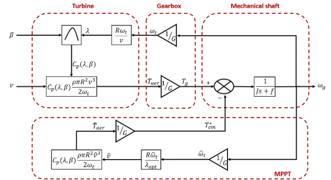
Fig. 7. Wind turbine block diagram with MPPT
