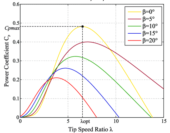
Fig. 2. Power coefficient curves
