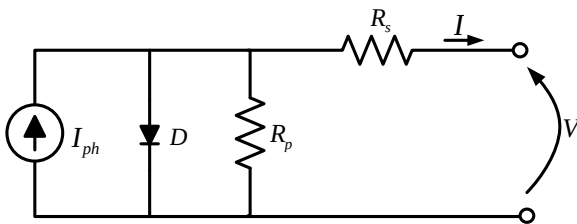
Fig. 1. Photovoltaic cell equivalent circuit.
