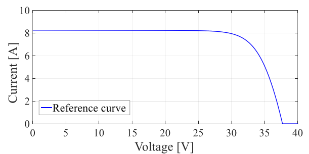
Fig. 4. PV module characteristic I-V curve used as parameter input of the DE algorithm.
