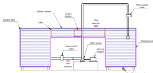
Fig 1. General configuration design of the experimental installation
