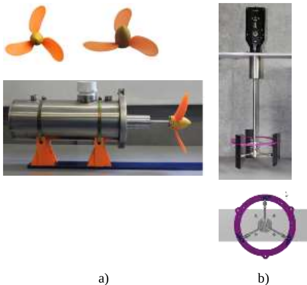
Fig. 5. a) Propeller hydrokinetic turbine, b) H-Darrieus hydrokinetic turbine
