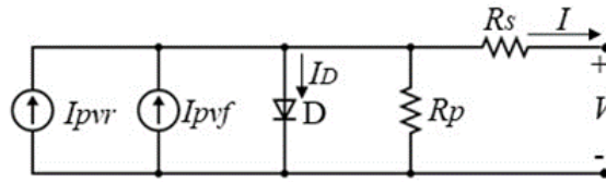
Fig. 3. Real single-diode PV cell model
