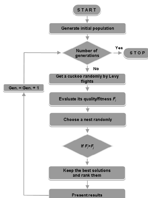
Fig. 1. Cuckoo search algorithm main steps
