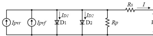
Fig. 4. Two-diode PV cell model
