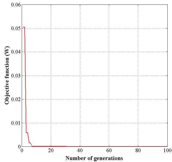
Fig. 6. Objective function change during the CSA search for real single-diode model at 1000 W/m 2
