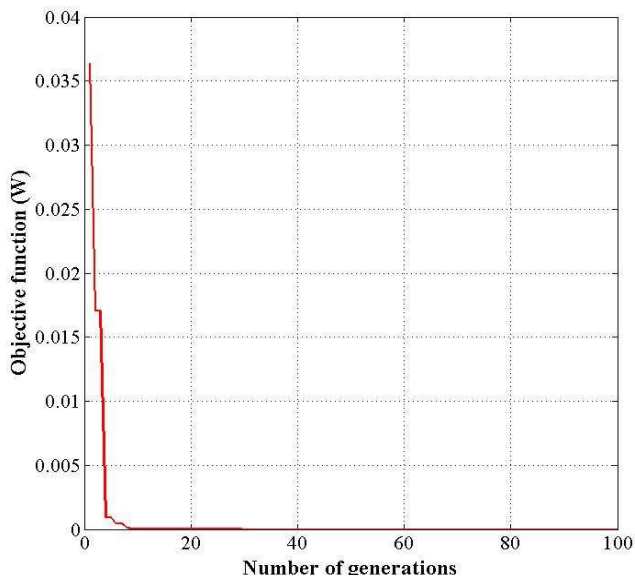
Fig. 5. Objective function change during the CSA search for ideal single-diode model at 1000 W/m 2
