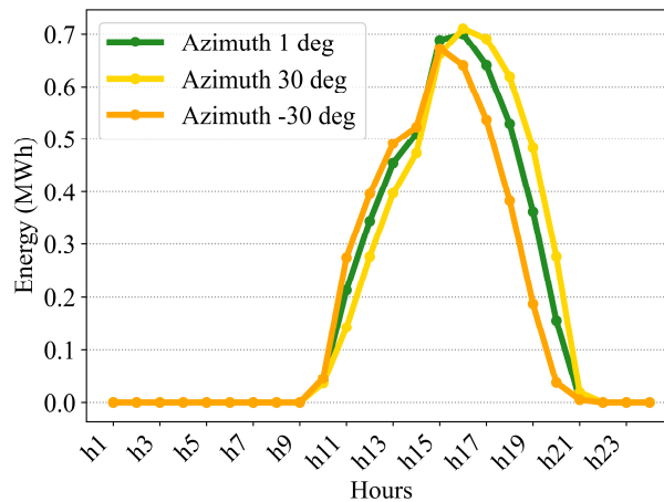
Fig.3. Hourly PV production of 1MWp at Seville 15 th September for Azimuth angles facing south, East (-30°) and west (30°).
