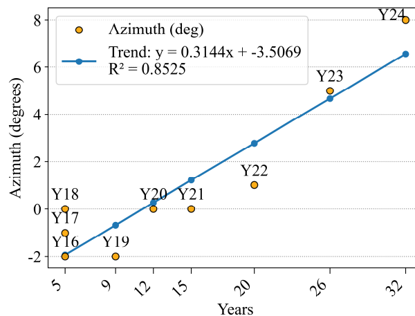
Fig. 6. Evolution of the azimuth angles and PV installed capacity.
