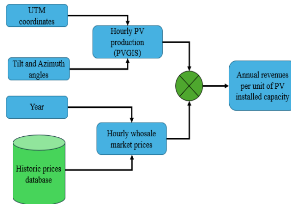
Fig. 1. Determination of annual revenues for a given year and PV panel orientation.
