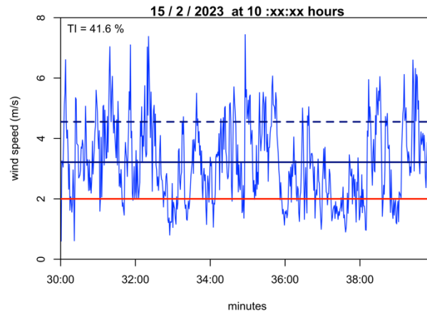
Fig.3. 10-minute segment of wind speeds recorded at a sampling rate of 1 Hz. Solid dark blue line: 10-min mean; solid red line: assumed cut-in wind speed of device; dashed blue line: assumed rated wind speed of device.
