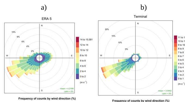
Fig.2. Wind roses, a) for the long-term ERA5 climatology, b) for the local anemometer.
