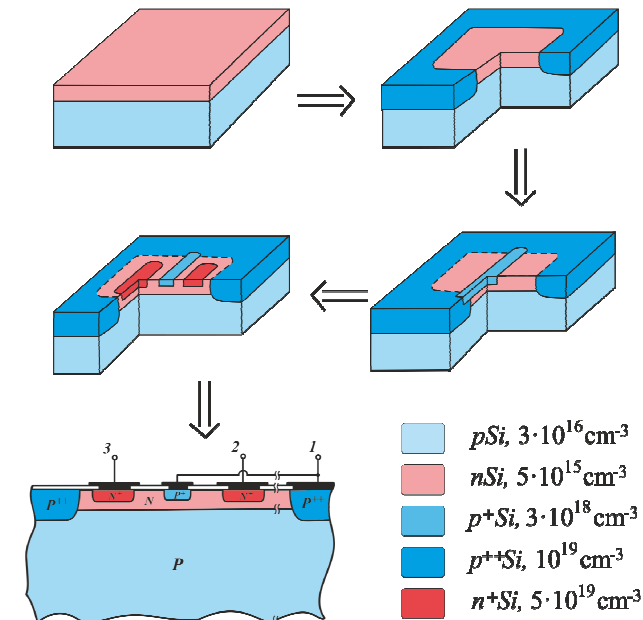
Fig. 1. Proposed diode temperature sensor and its fabrication steps.
