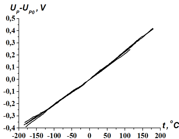
Fig. 4. The temperature response curves (TRCs) of 10 proposed diode temperature sensor samples
