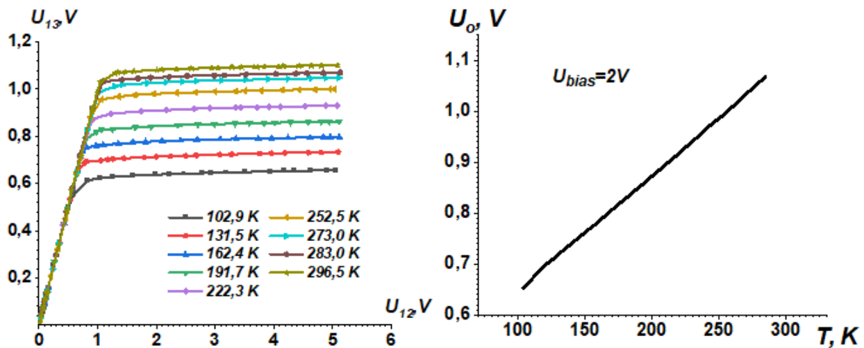
Fig. 3. Typical measured output voltage ( U_{13} ) versus bias voltage ( U_{12} ) characteristics at different temperatures (a) and the temperature response curve (TRC) of proposed diode temperature sensor
