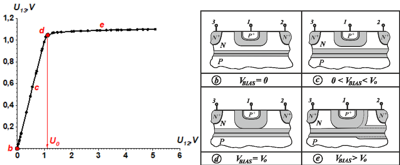
Fig. 2. Typical measured output voltage ( U_{13} ) versus bias voltage ( U_{12} ) characteristics of proposed diode temperature sensors (a) and the structural diagrams (b-e) of the device under study at various bias voltages
