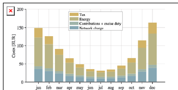
Fig.2. Cost structure of electricity in the case of the old network charge calculation system without a balcony solar power plant
