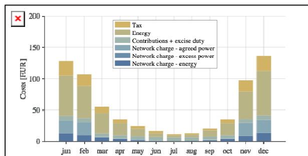
Fig.8. Cost structure of electricity in the case of the new network charge calculation system with a balcony solar power plant and a battery storage system
