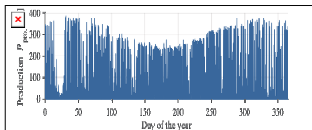
Fig.4. Electricity generation of the balcony solar power plant for the analyzed household consumer
