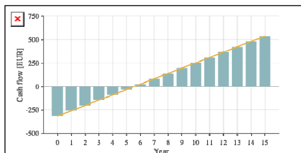
Fig.9. Payback period of the investment in the balcony solar power plant under the new network charge calculation system
