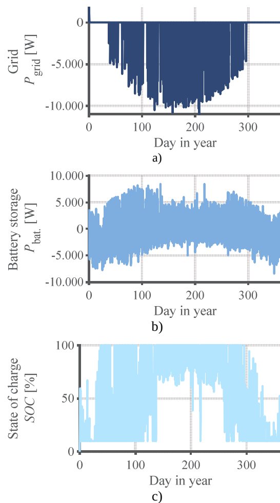
Fig. 2. Power flow into/from grid and battery storage, State of charge for battery storage
