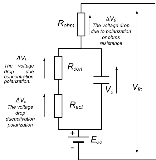
Fig.2. Equivalent electrical circuit model of PEMFC
