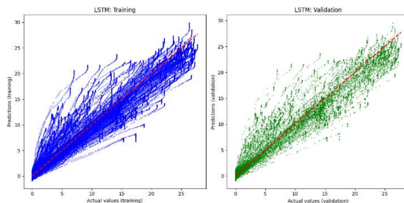
Fig. 2. Accuracy of the LSTM model in the training set: Predictions versus actual values (left). And accuracy of the LSTM model in the validation set: Predictions versus actual values (right).
