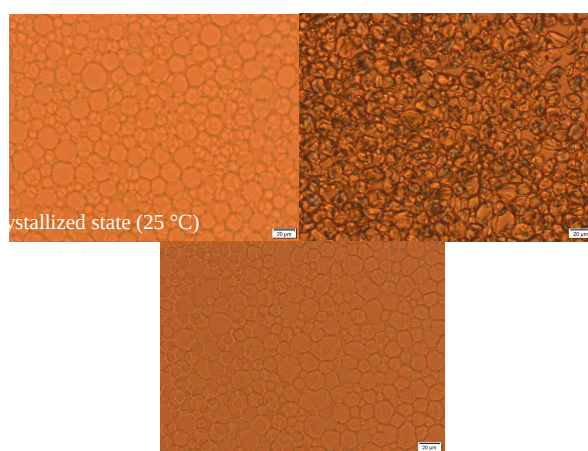
Fig. 2 Optical microscopy images of PCME (40%) emulsion at (a) 80 °C, (b) 25 °C, (c) 80 °C
