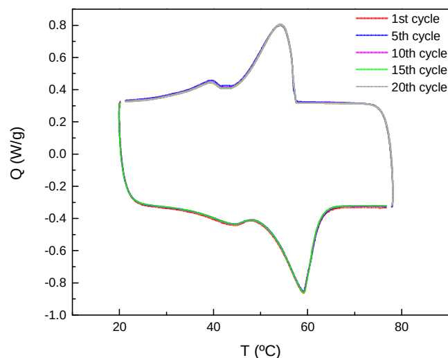
Fig. 3 MSDC curves for emulsions after thermal cycling
