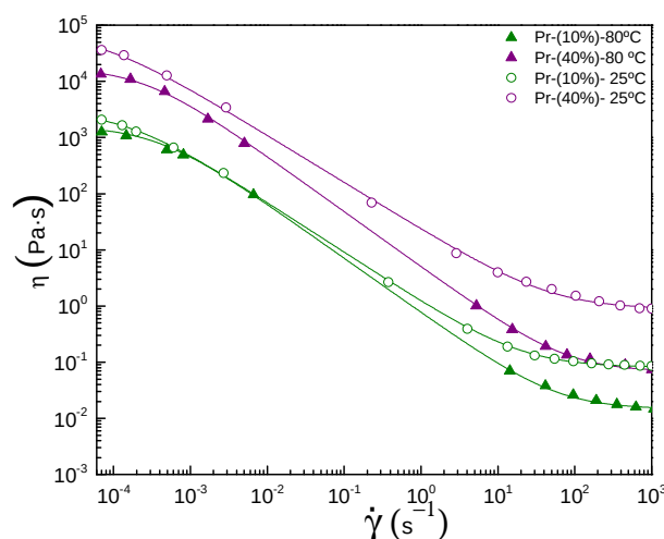
Fig. 1 Flow curves for PCM emulsions
