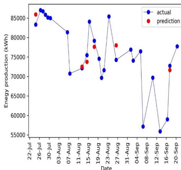
Fig. 2. Daily energy production measured (blue dots) and predicted (red dots) for the study period, using the 4 most important features.
