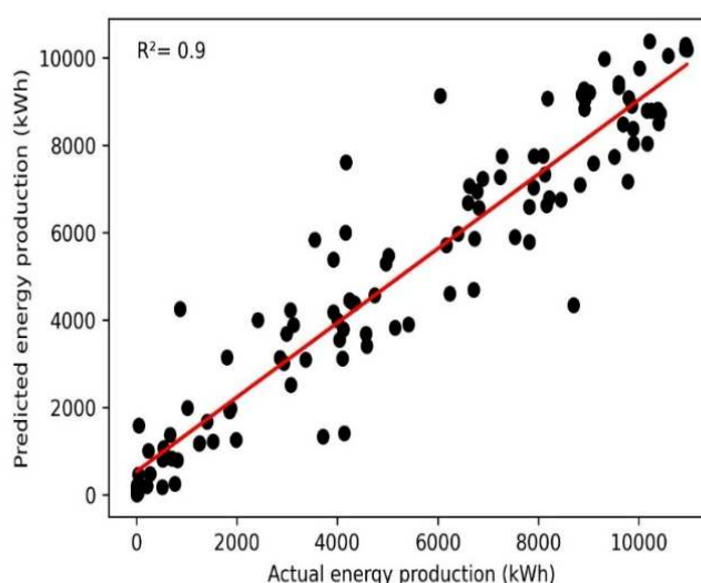
Fig. 3. Scatter plot of predicted v.s. actual hourly energy production using the 10 most important features.
