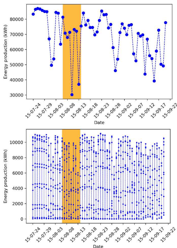
Fig. 1. Daily (top) and hourly (bottom) total energy production for the study period. The African dust episode from 6th to 14th August is shaded in orange.
