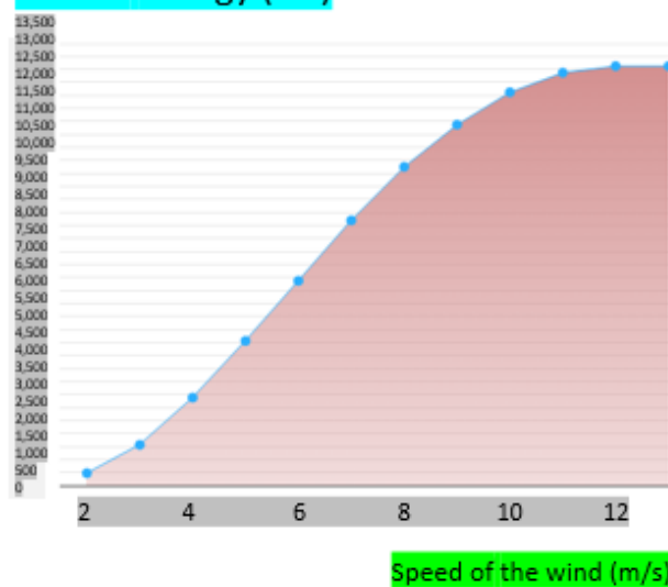
Fig.3. Power and Annual Energy as function of wind speed
