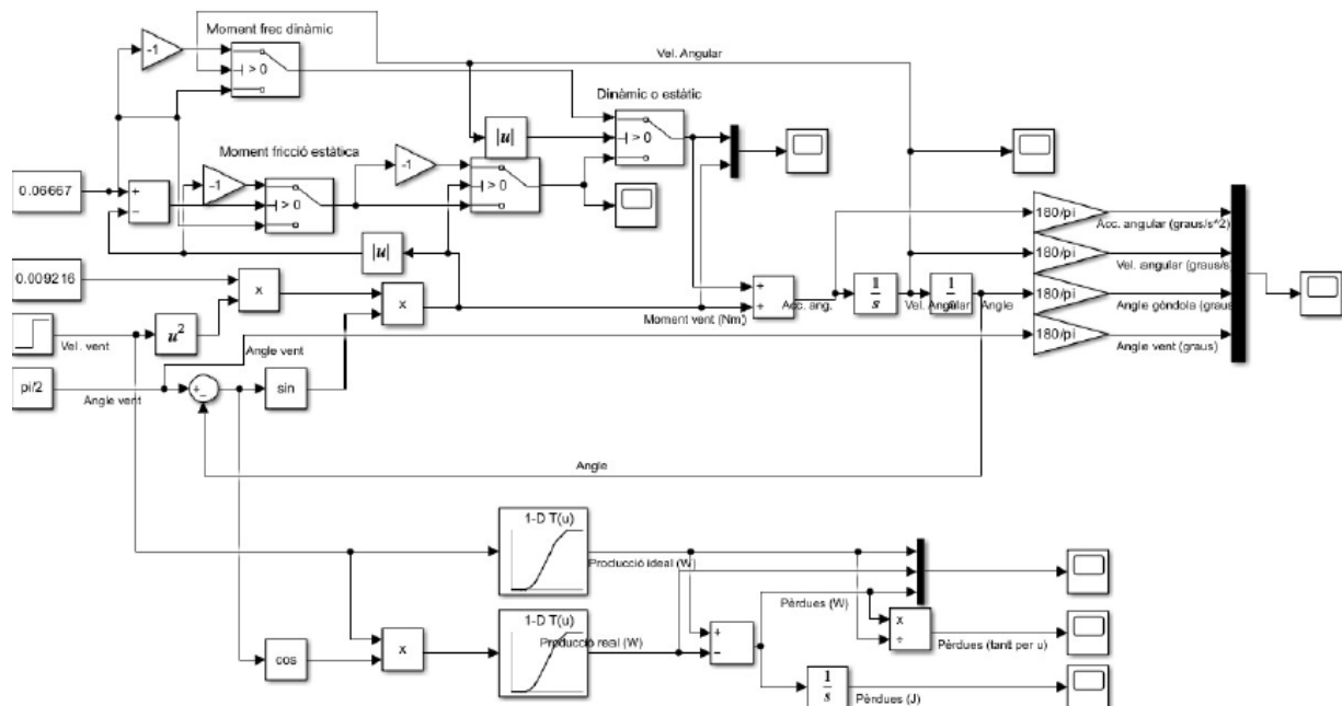
Fig. 7. The simulated model
