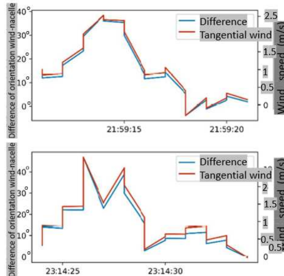
Fig. 6. Experimental data from Eco-granja Vilà.
