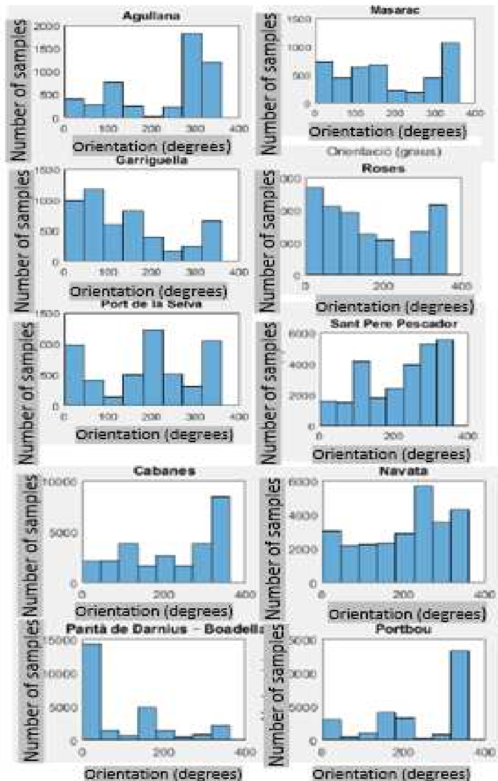
Fig. 4. Wind orientation for the studied locations
