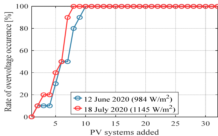
Fig. 3. Rate of overvoltage occurrence at any consumer bus for different numbers of PV systems added.
