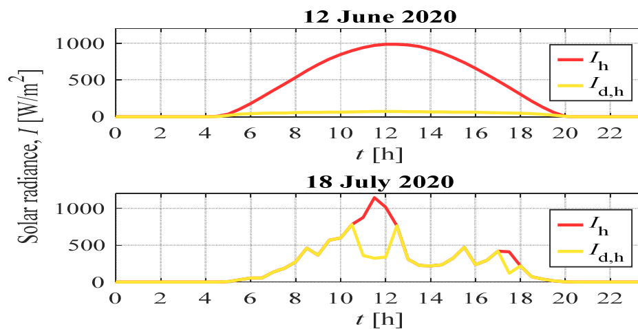
Fig. 1. Daily course of global and diffuse solar radiation on 12. June 2020 and 18. July 2020.
