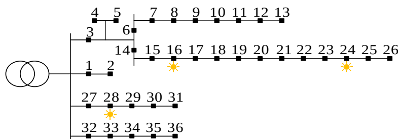
Fig. 2. Grid topology of the studied feeder with annotations of locations of existing PV systems in yellow marks.
