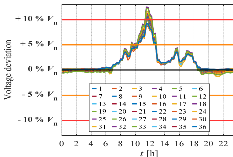
Fig. 6. Voltage deviation for all consumer buses, with six added PV systems, on 18 July 2020.
