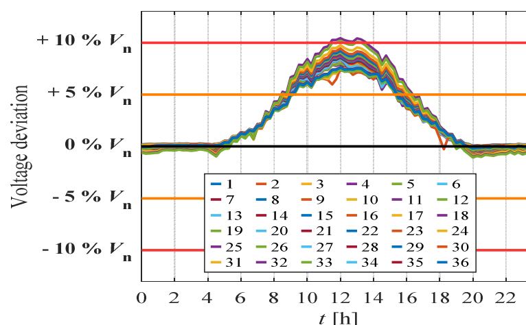
Fig. 4. Voltage deviation for all consumer buses, with six added PV systems, on 12 June 2020.
