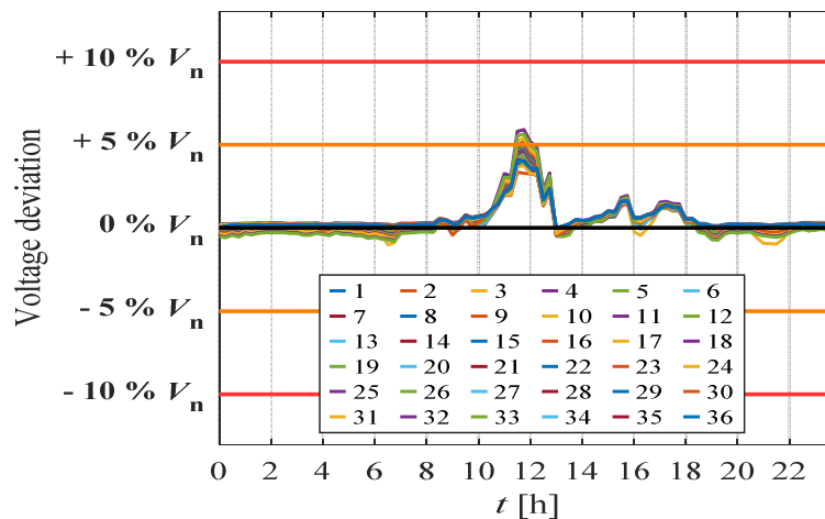
Fig. 7. Voltage deviation for all consumer buses, with added energy storage systems to all PV systems, on 18 July 2020.
