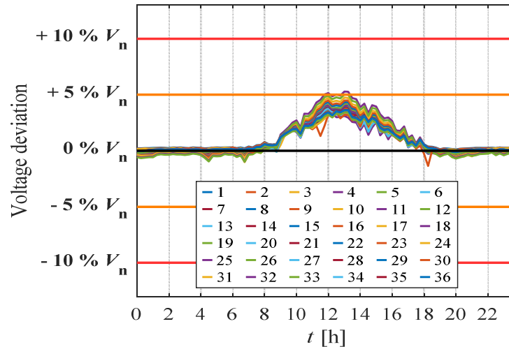
Fig. 5. Voltage deviation for all consumer buses, with added energy storage systems to all PV systems, on 12 June 2020.
