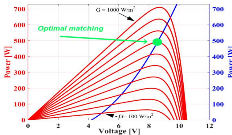
Figure 6. Power versus voltage curves of the PV configuration with eight arrays parallel connected and load curve.
