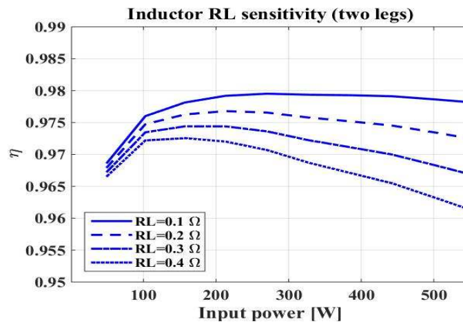
Figure 13. Efficiency calculated for different values of the Inductor parasitic resistance.
