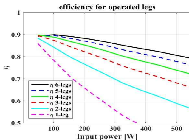
Figure 7. Efficiency calculated with eight parallel connected arrays.
