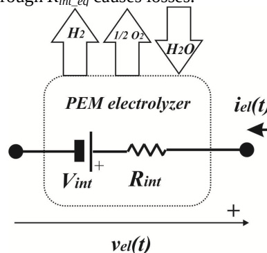
Figure 2. Circuitual model of the electrolyzer.
