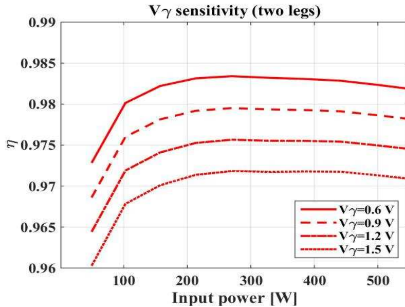
Figure 11. Efficiency calculated for different values of the diodes drop voltage
