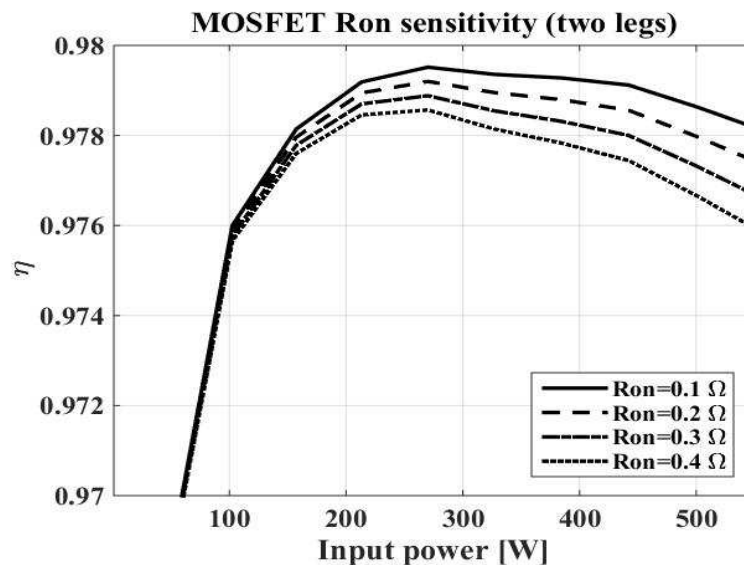
Figure 12. Efficiency calculated for different values of the MOSFET conduction resistance.
