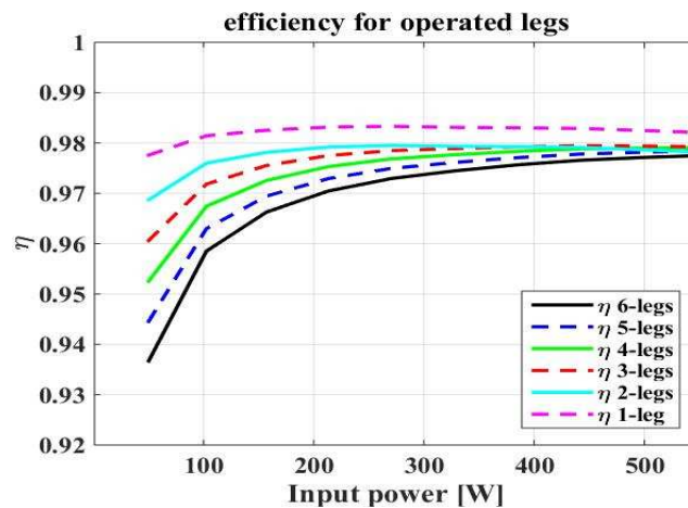
Figure 10. Efficiency calculated with eight arrays connected in series.
