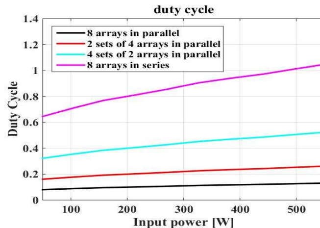
Figure 12. Duty cycle of the converter versus power for different PV source configurations.
