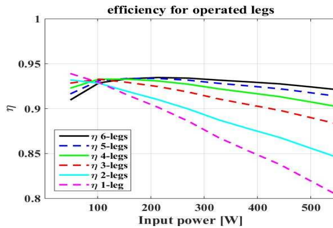
Figure 8. Efficiency calculated with a series connection of two sets of four arrays parallel connected.
