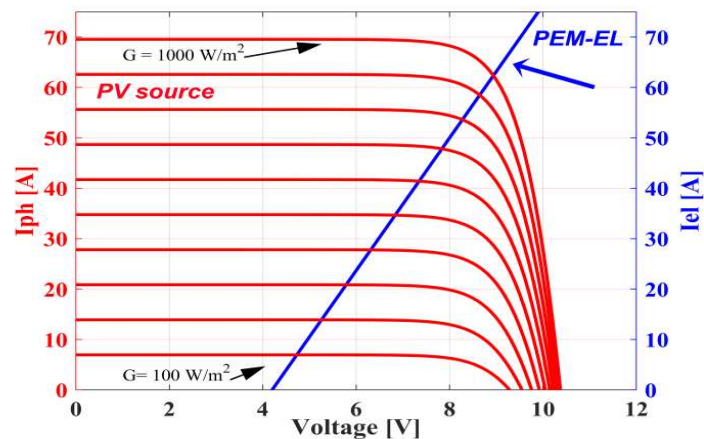
Figure 5. Current versus voltage curves of the PV configuration with eight arrays parallel connected and load curve.
