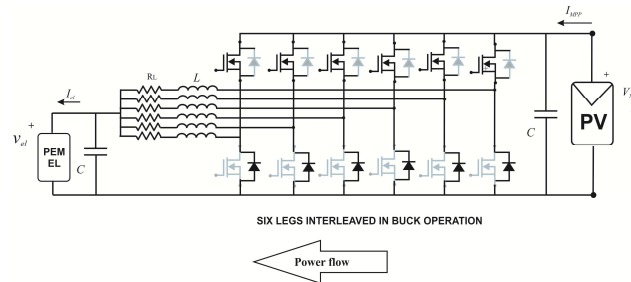
Figure 3. Electric scheme of the six legs converter in Buck operation
