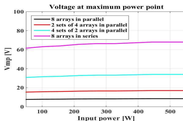
Figure 11. Voltage at the maximum power point versus power for different PV source configurations.
