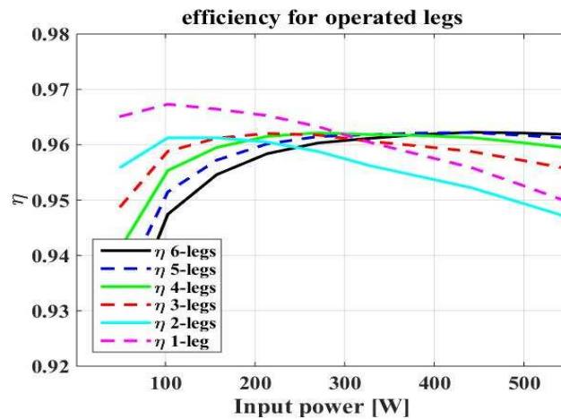
Figure 9. Efficiency calculated with a series connection of four sets of two arrays parallel connected.
