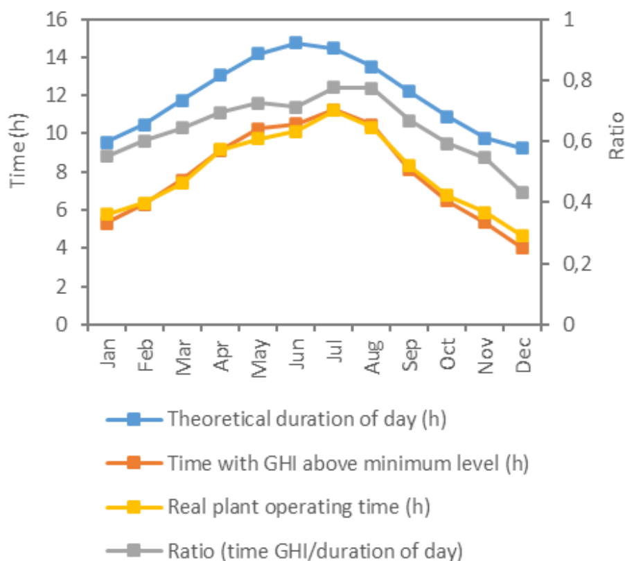
Fig. 2. Duration of tests and solar radiation.
