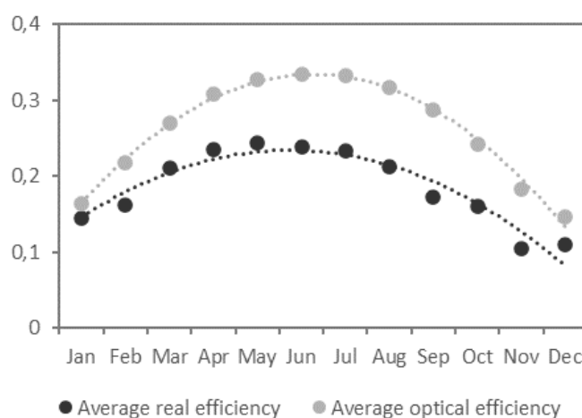
Fig. 4. Real and optical efficiency.
