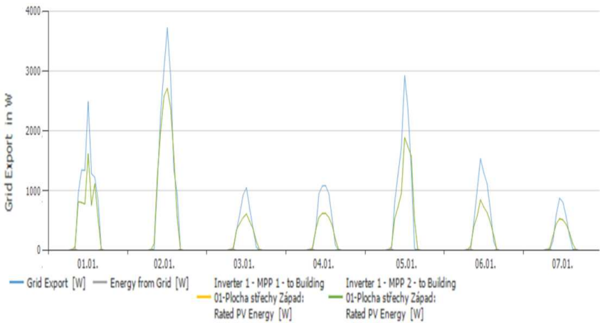
Fig 5.: Power generation before reaching the optimal values of the similarity criteria (PV*SOL Premium).
