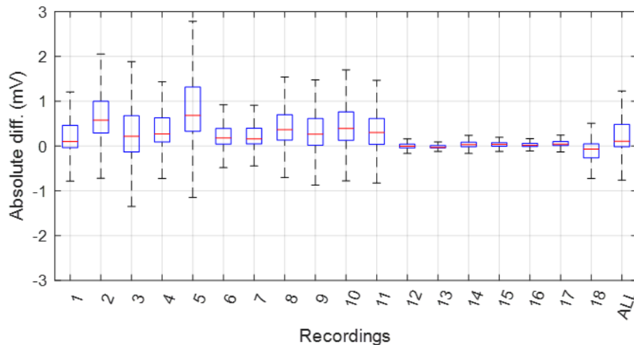
Fig. 5. Absolute values of the differences between the QP spectra of CISPR16 and Light QP
