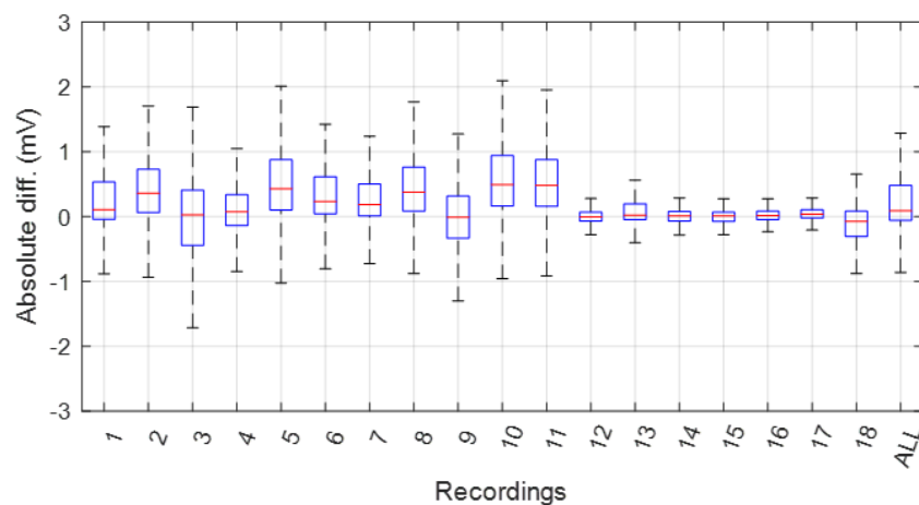
Fig. 6. Absolute values of the differences between the QP results of CISPR16 and Statistical QP.
