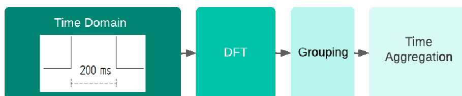
Fig. 1. Main steps of the IEC 61000-4-7 method
