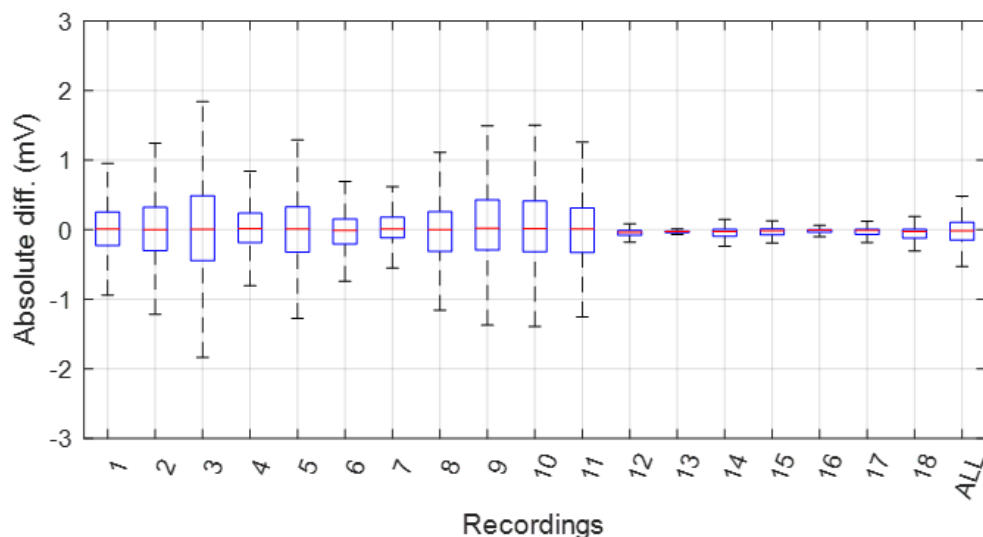
Fig. 4. Absolute values of the differences between the RMS spectra of IEC 61000-4-7 and RM-A
