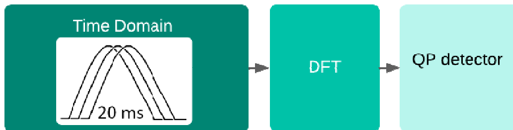
Fig. 3. Main steps of the CISPR-16 method
