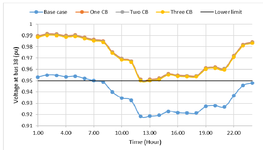
Fig. 10. The voltage profile of bus 38 in case 3
