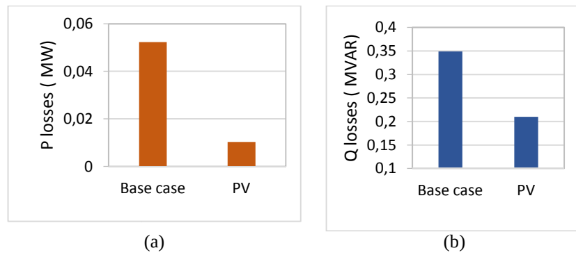
Fig. 7. The power losses of case 2, (a) total active power losses; (b) total reactive power losses
