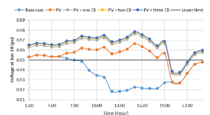
Fig. 14. The voltage profile of bus 38 in case 4
