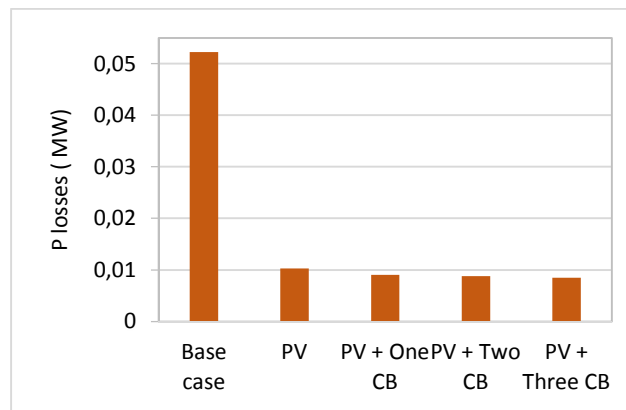
Fig. 12. The total active power losses of case 4
