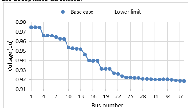
Fig. 3. Voltage profile of the base case
