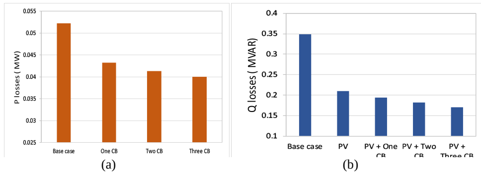
Fig. 9. The power losses of case 3, (a) total active power losses; (b) total reactive power losses
