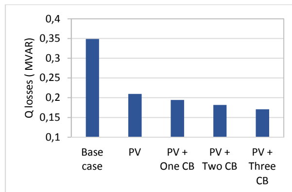
Fig. 13. The total reactive power losses of case 4
