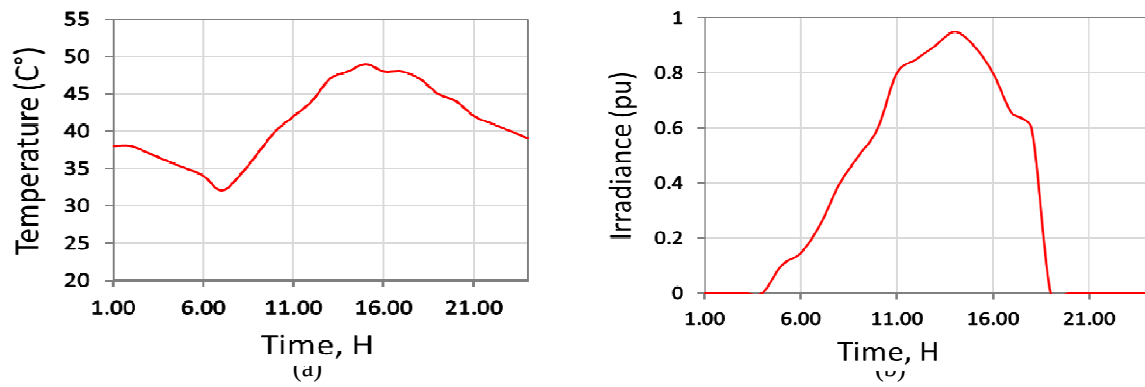
Fig. 4. (a) daily temperature curve; (b) daily irradiance shape
