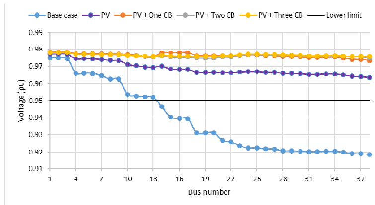
Fig. 11. Voltage profile of the case 4 (integration of CBs with PV arrays)
