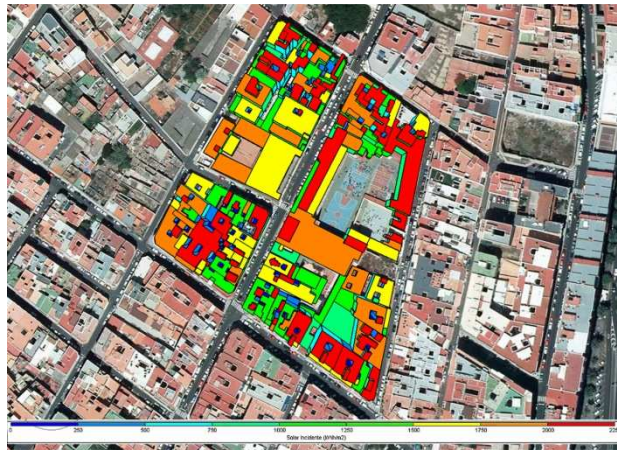
Fig.7. Aerial photo of the study area in El Toscal, with incident irradiation normalized by roof surface ( \text{kWh/m}^2 \cdot \text{year} ) with the PVGIS climate file.
