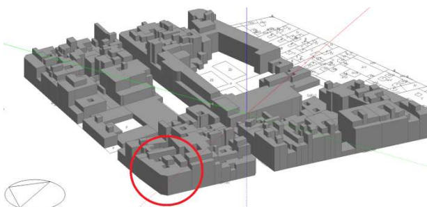
Fig.3. Set of building blocks modelled in DesignBuilder in the El Toscal neighbourhood and building selected for the simulated photovoltaic installation framed in a circle.
