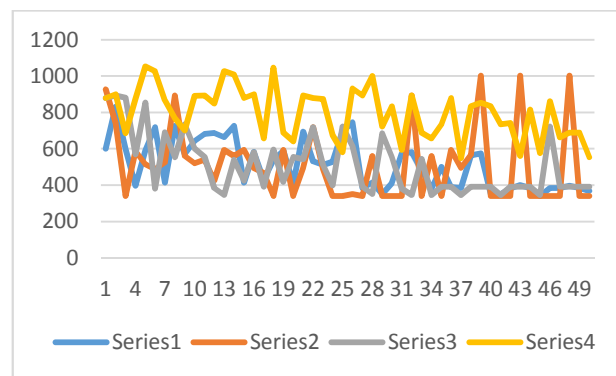
Fig.5. Tardiness results for the penalty method II
