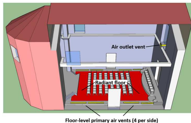
Fig. 3. DesignBuilder 3D Model – Case 2
