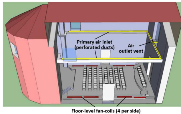
Fig. 2. DesignBuilder 3D Model – Case 1
