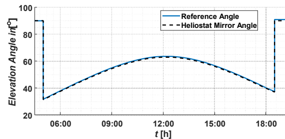
Figure 10. Reference and tracking angle for elevation angle with heliostats mirror angles on Jun. 15 th , 2020.
