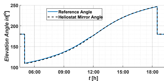
Figure 9: Reference and tracking angle for azimuth angle with heliostats mirror angles on Jun. 15 th , 2020.
