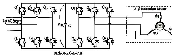
Figure 6. Back-to-back converter for three-phase Induction Motor
