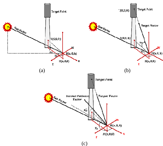
Figure 2. The dimensions for (a) sun elevation and azimuth angles, (b) tower elevation and azimuth angles, and (c) heliostat elevation and azimuth angles.
