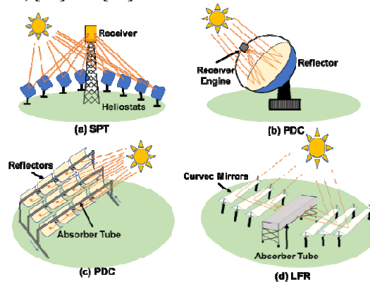
Figure 1. Different CSP topologies
