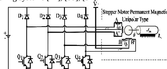
Figure 5. Power Circuit of unipolar PM Stepper Motor Model
