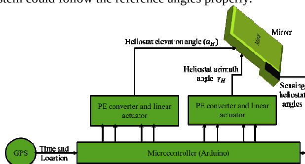
Figure 7. Block diagram of dual-axis solar tracking system
