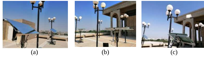
Figure 8. The proposed prototype of the automatic dual-axis solar tracking unit.
