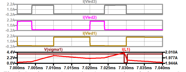
Fig. 6. Steady-state (up to down) current through the stages C (grey), B (violet), A (brown); current through the coil (red), output of the controller (black): low input voltage.
