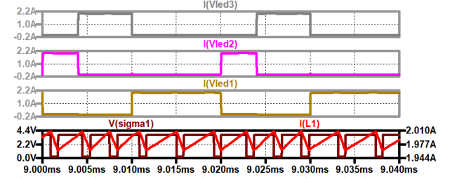
Fig. 7. Steady-state (up to down) current through the stages C (grey), B (violet), A (brown); current through the coil (red), output of the controller (black): high input voltage.
